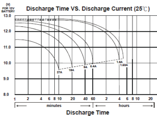
Constant Power Discharge Characteristics (25°C) [Watt]
